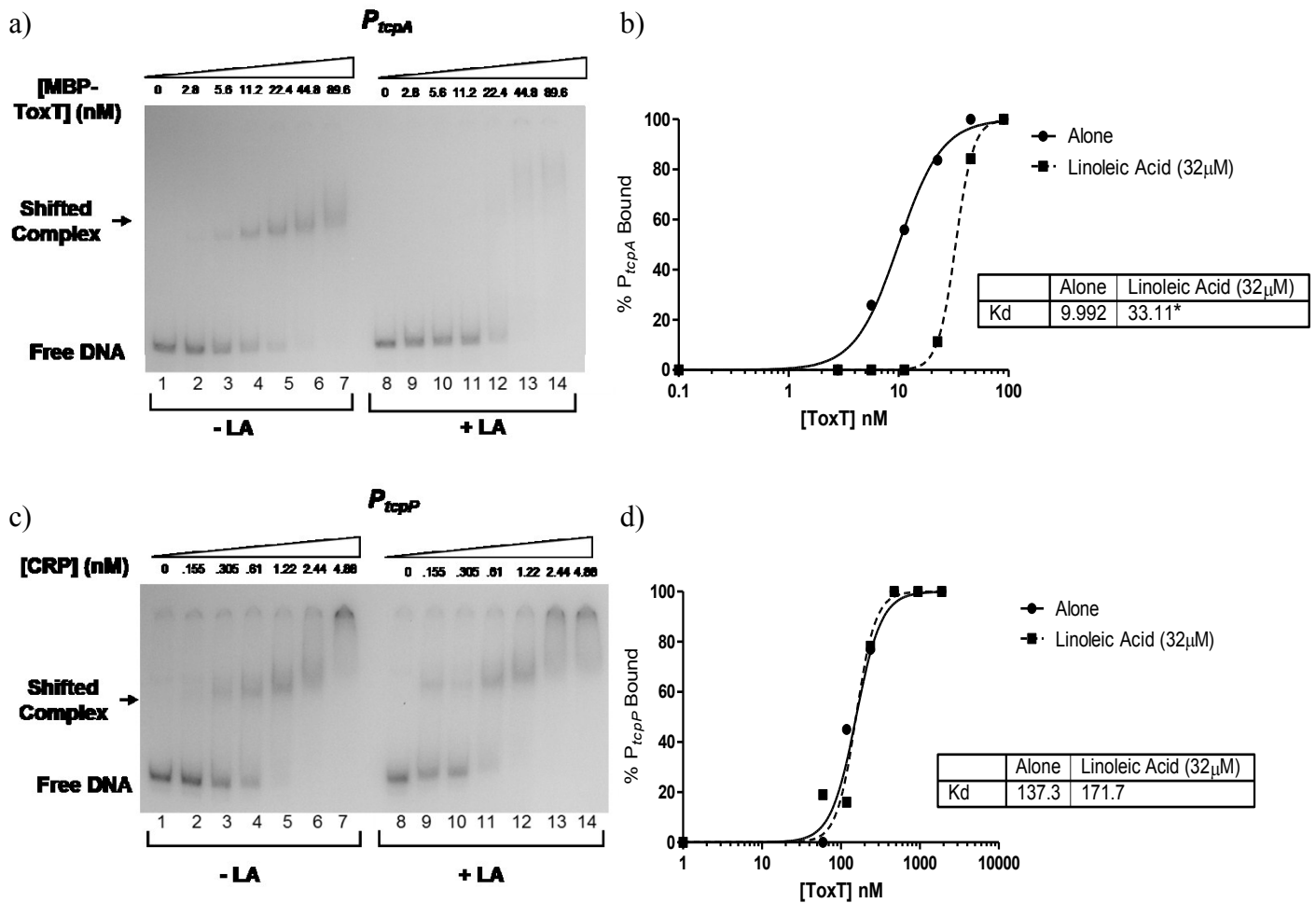
FIGURE 6. Linoleic acid decreases binding affinity of MBP-ToxT to P_{tcpA} . MBP-ToxT binding to P_{tcpA} was analyzed using EMSA. (A) Binding reactions between MBP-ToxT and P_{tcpA} in lanes 1-7 were conducted in the absence of linoleic acid. Lanes 8-14 were incubated in the presence of 32µM linoleic acid. Lanes 1 and 8 contained P_{tcpA} DNA in the absence of MBP-ToxT. Subsequent lanes contained a titration of MBP-ToxT with concentrations labeled in the figure. (B) Binding curve for the autoradiograph shown in (A). Densitometry of autoradiograph was performed with ImageJ software. Circles represent percent P_{tcpA} bound by MBP-ToxT in the absence of linoleic acid. Solid line corresponds to the binding curve for MBP-ToxT. Squares and dashed line represent percent bound and binding curve, respectively, in the presence of linoleic acid. (C) Autoradiograph of EMSA showing titration of MBP-CRP bound to P_{tcpP} with DMSO (Lanes 1-7) and linoleic acid (Lanes 8-14). (D) Binding curves with and without linoleic acid with K_d . Autoradiographs of EMSAs presented are representative of three or more independent experiments. K_d for each condition is inset and significant difference between the best-fit values of each data set is denoted by * ( p < 0.0001 ).
